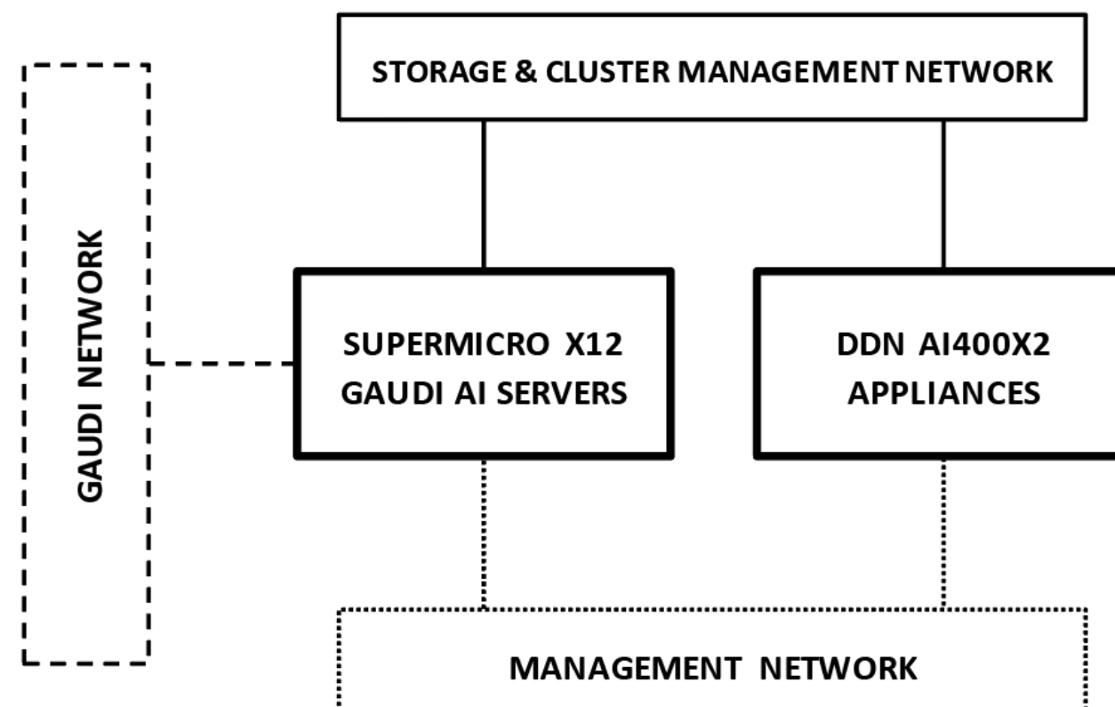
Figure 10. Overview of the network architecture
