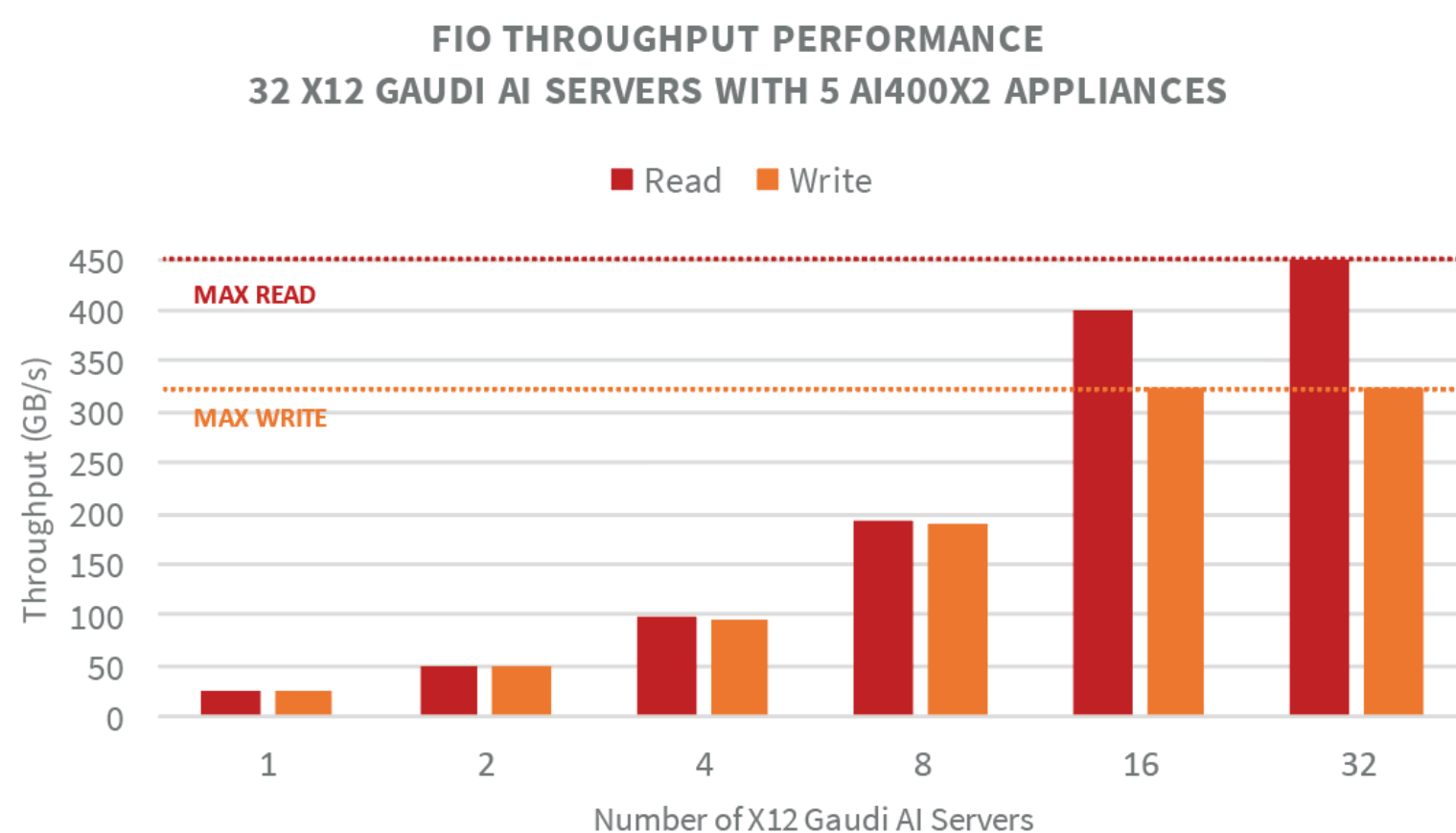
Figure 24. FIO throughput scaling with a very large number of X12 Gaudi AI servers
