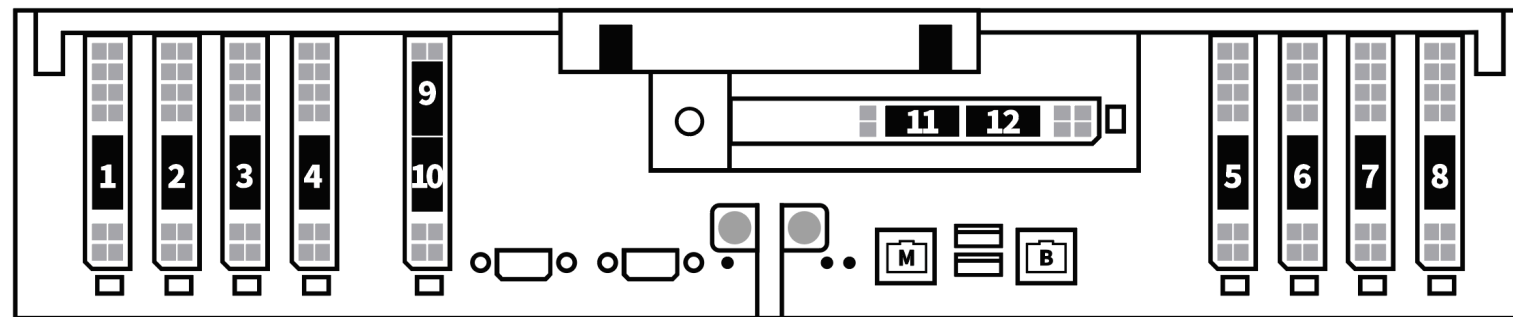
Figure 9. Recommended DGX A100 system network port connections.
