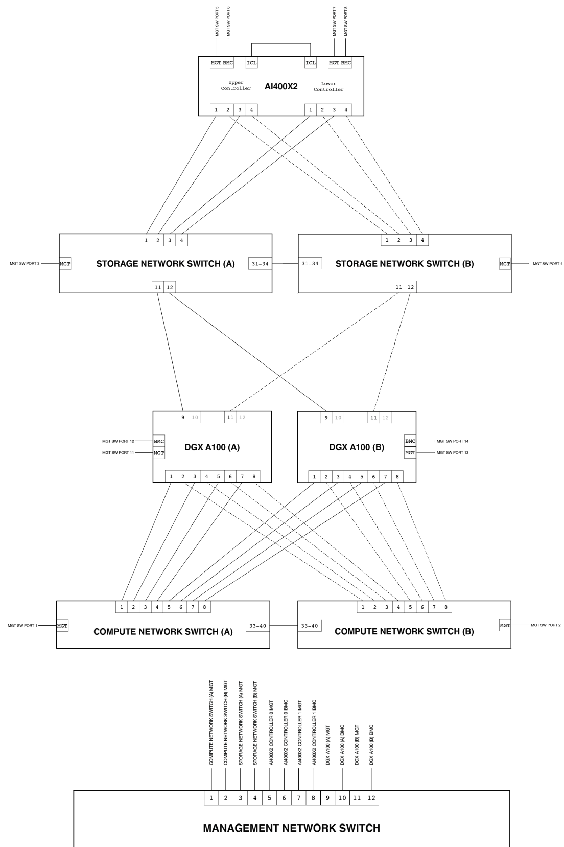
Figure 12. DDN A 3 i POD network diagram with two DGX A100 systems.
