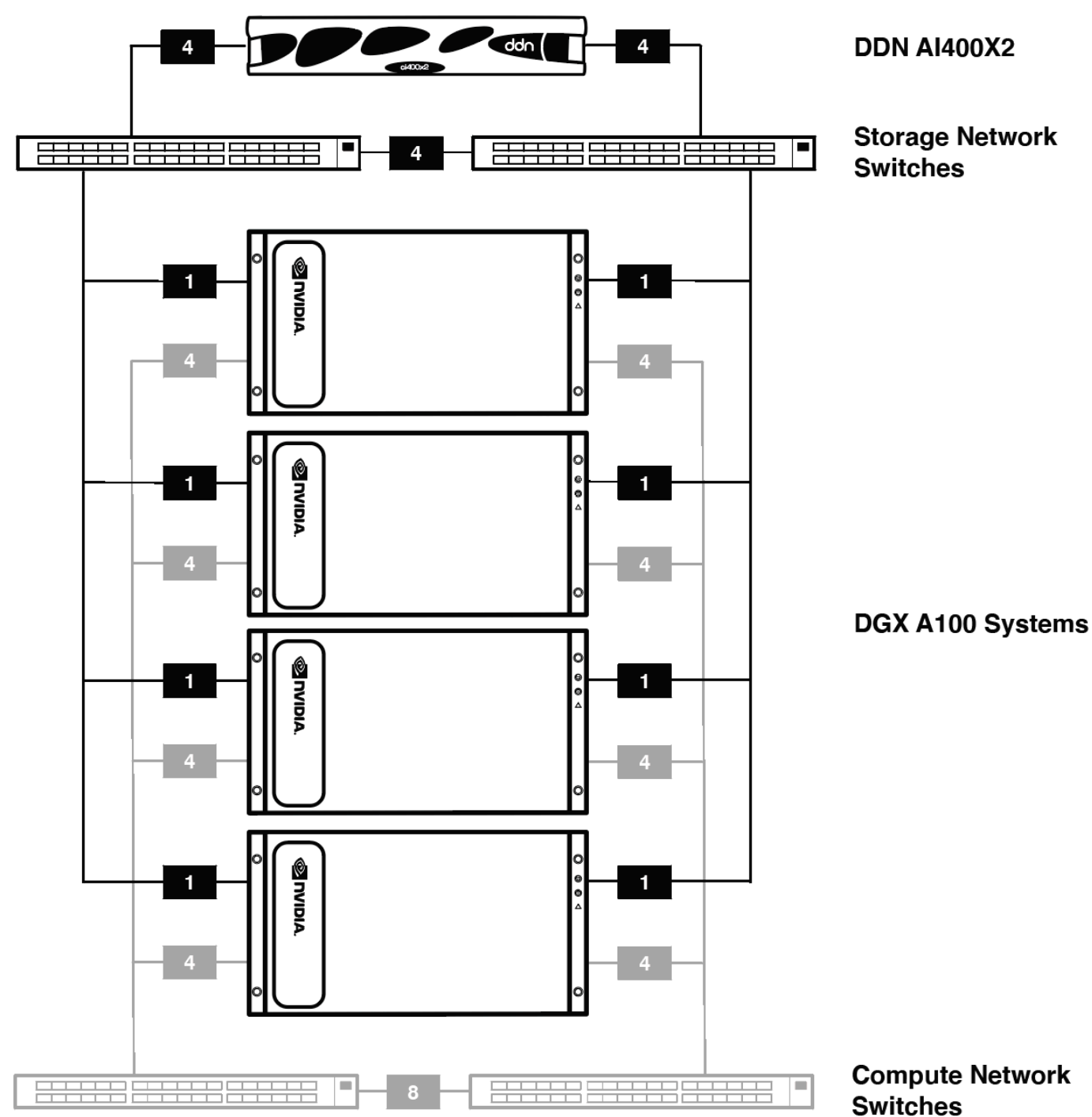
Figure 13. DDN A 3 I POD reference architecture with four DGX A100 systems (management network not shown).
