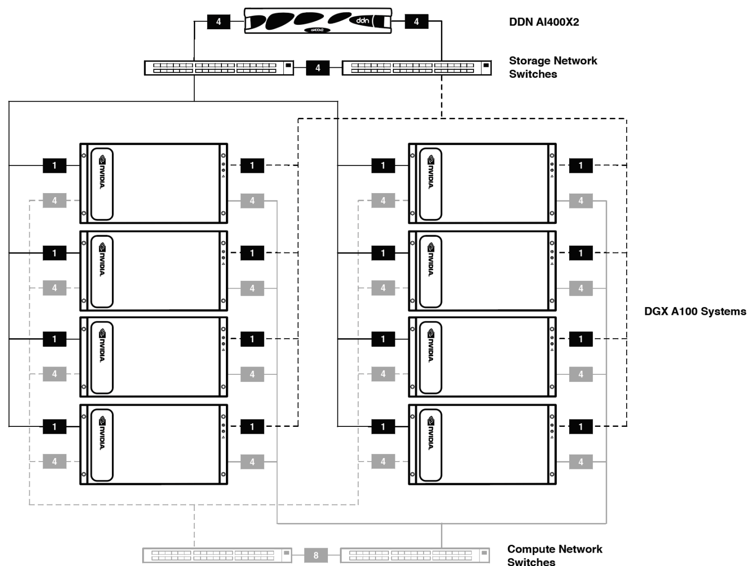
Figure 18. Test environment with eight DGX A100 system and one AI400X2 (management network not shown).
