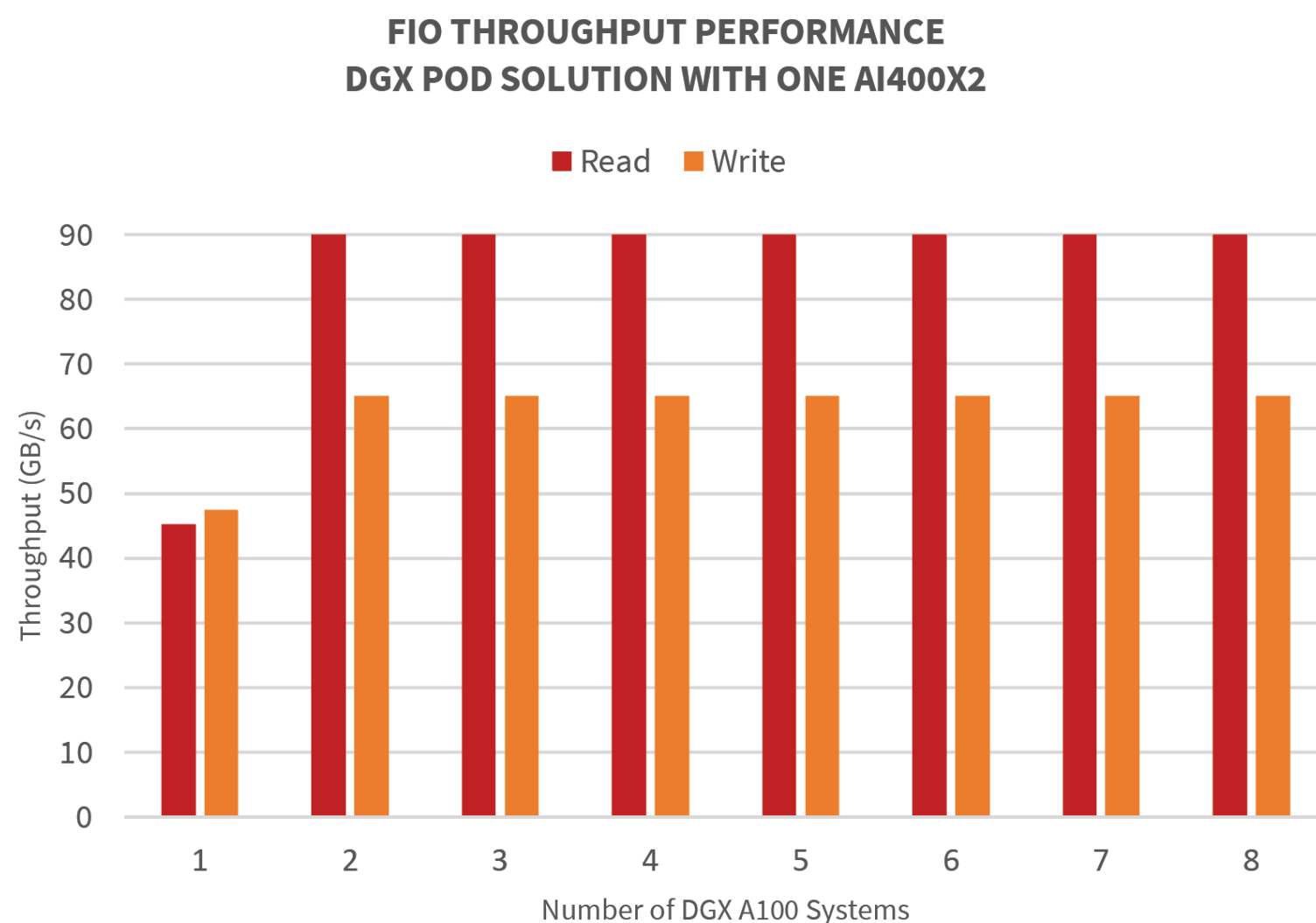
Figure 19. FIO throughput with scaled DGX POD configurations.
