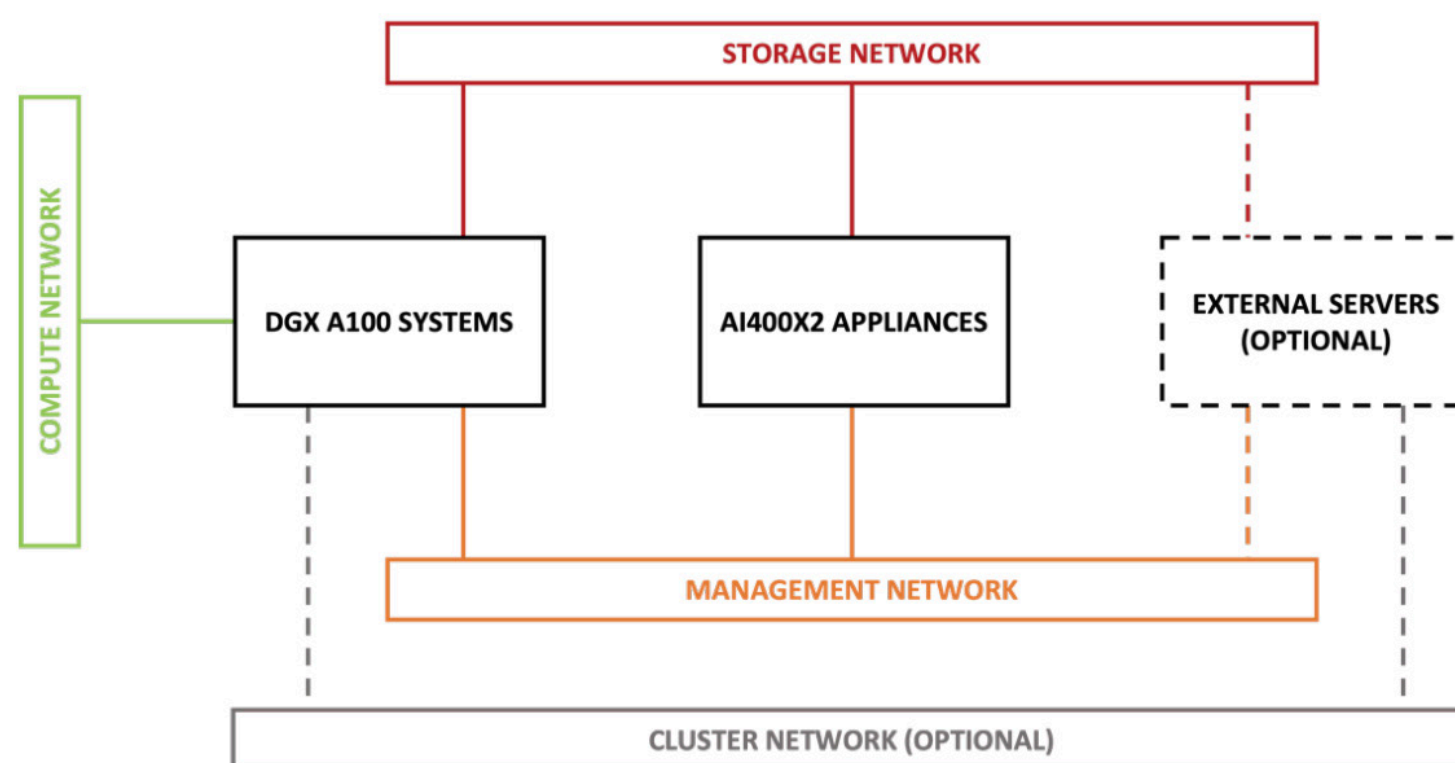
Figure 8. Overview of the DGX POD network architecture.
